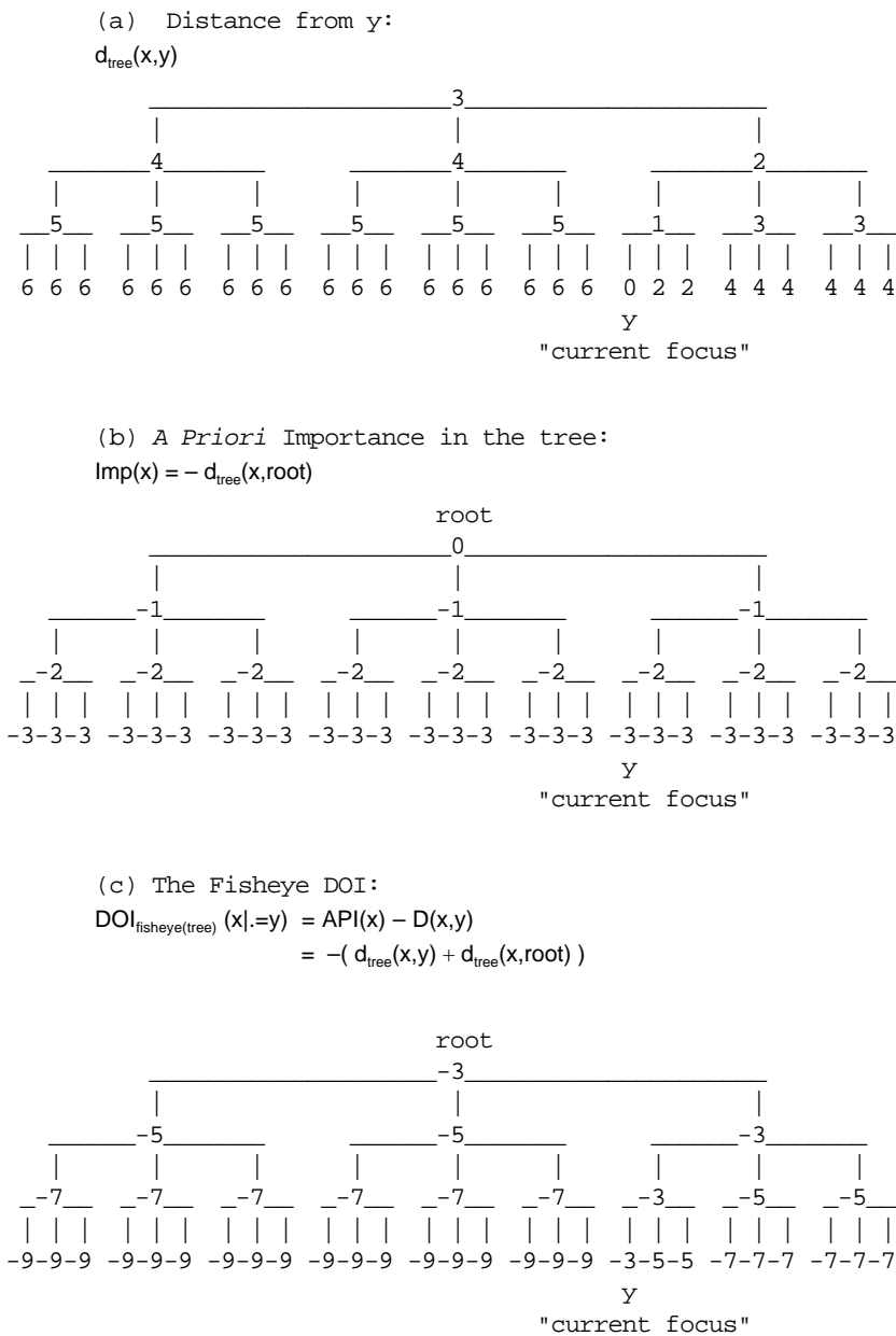
Figure 1. Distance, A Priori Importance and the Fisheye DOI for a rooted tree.
