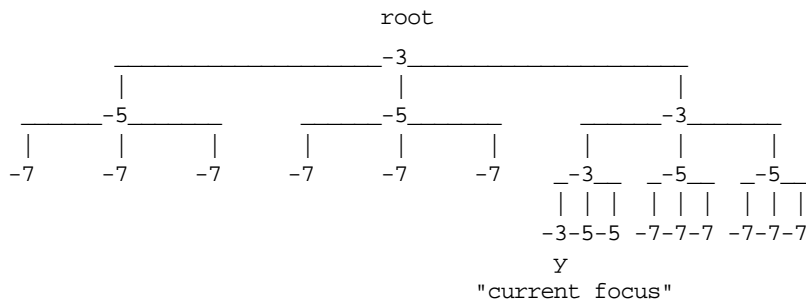
Figure 2. Zero-order, first-order and second-order fisheye views for a tree.
