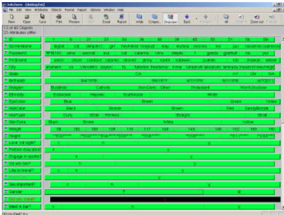
Figure 1b. This screenshot shows one possible way for solving the same problem in InfoZoom, specifically in its overview mode. After clicking at, and thereby zooming into, the “Yes” entries in the attribute “Did you cheat?,” users can see from the length of the bars in the Gender category that females indicated more frequently having cheated than males.
